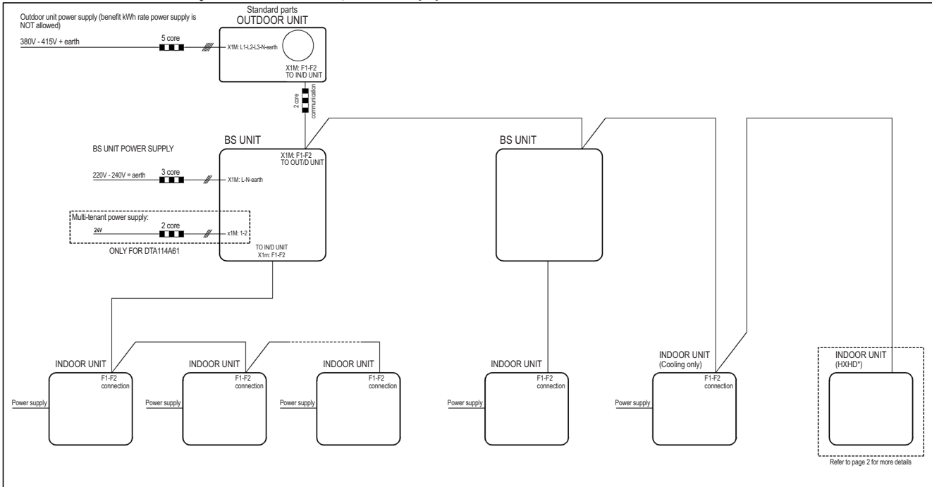
Electrical connection diagram
