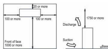
Required installation space
